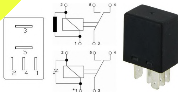
E020041 Micro-relais 12V 30/20A +diode
