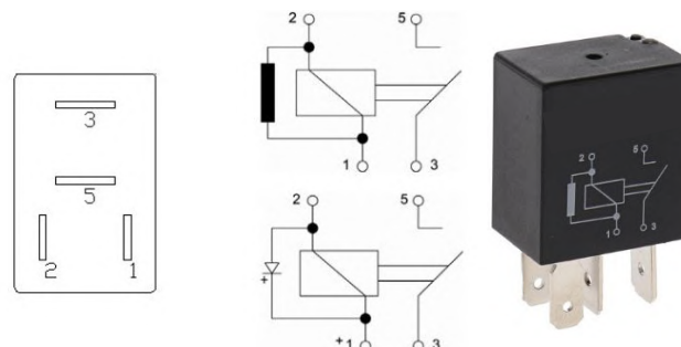
E020043 Micro-relais 12V 30A +diode
